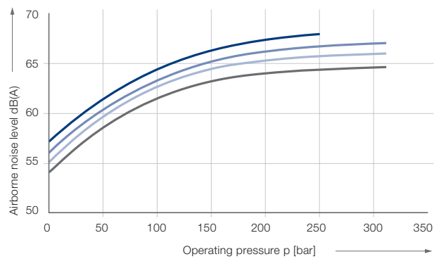
IPVA 5 – Airborne noise level (measuring location 1 m axial)
