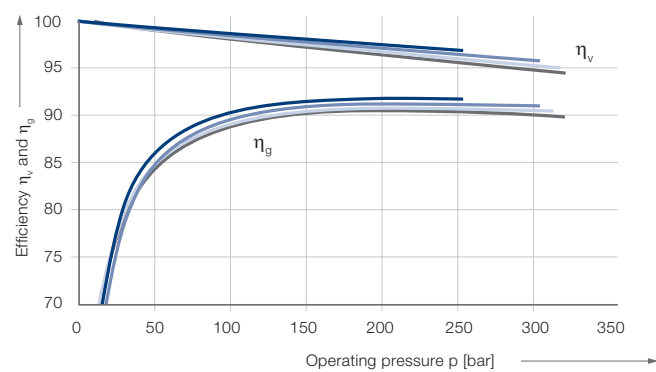
IPVA 6 – Efficiency \eta_v and \eta_g
