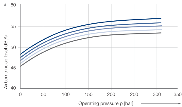
IPVA 3 – Airborne noise level (measuring location 1 m axial)
