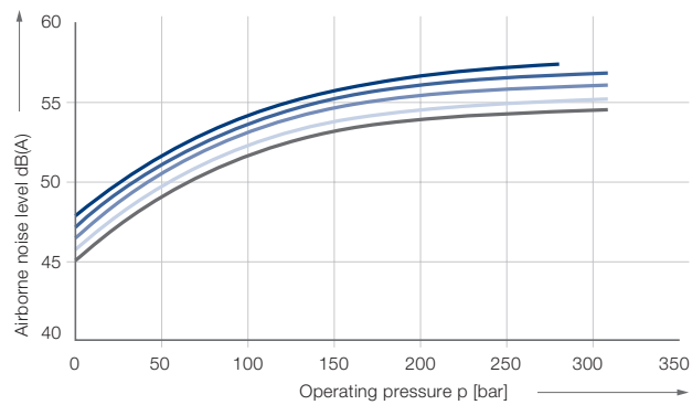
IPVA 4 – Airborne noise level (measuring location 1 m axial)
