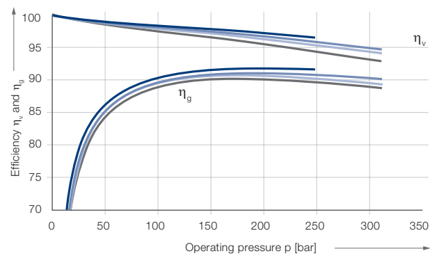
IPVA 5 – Efficiency \eta_v and \eta_g
