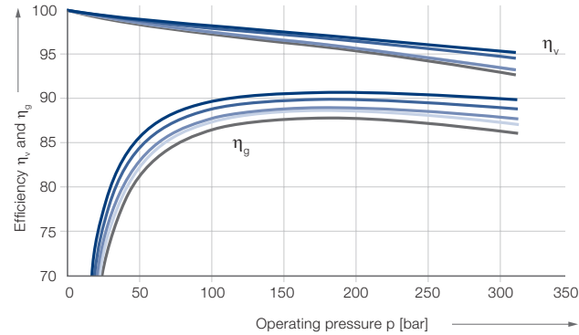
IPVA 3 – Efficiency \eta_v and \eta_g
