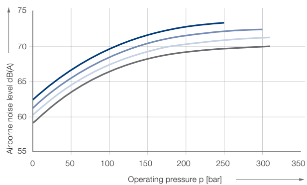
IPVA 6 – Airborne noise level (measuring location 1 m axial)
