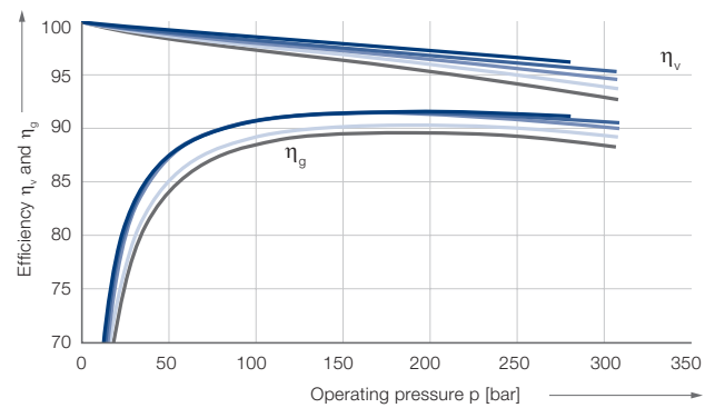
IPVA 4 – Efficiency \eta_v and \eta_g
